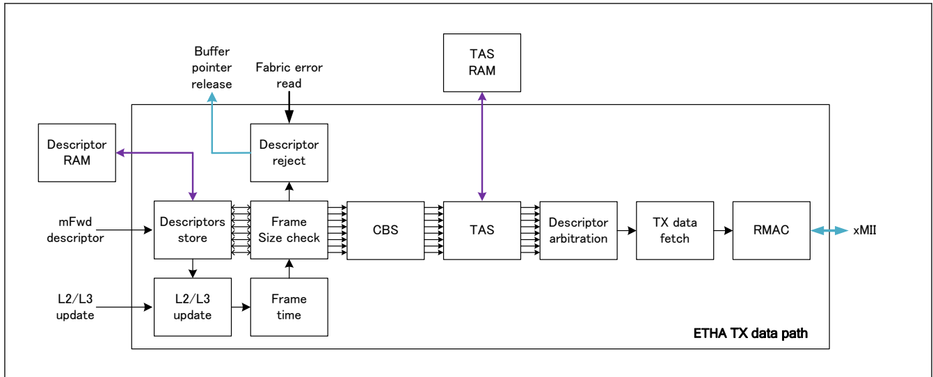
Figure 33.18 ETHA TX data path block diagram
